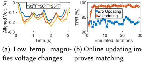
(a) Voltages collected in different scenarios (b) Matching results
