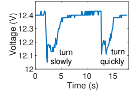
Fig. 16. Battery voltage varies with repetitions of operations.
